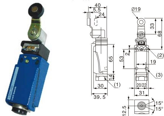
LL3XCDR2118P20 热塑滚轮摇杆
